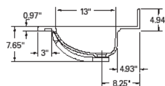
SIDE CROSS-SECTION
