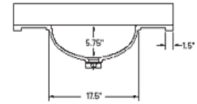
FRONT CROSS-SECTION
