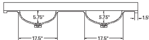
FRONT CROSS-SECTION
